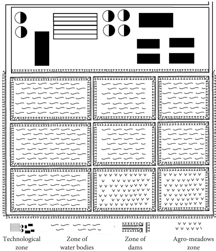
Fig. 2. Sketch of waste water treatment plants.
