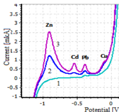
Fig. 1. Voltamperograms of the mushroom sample of ceps
